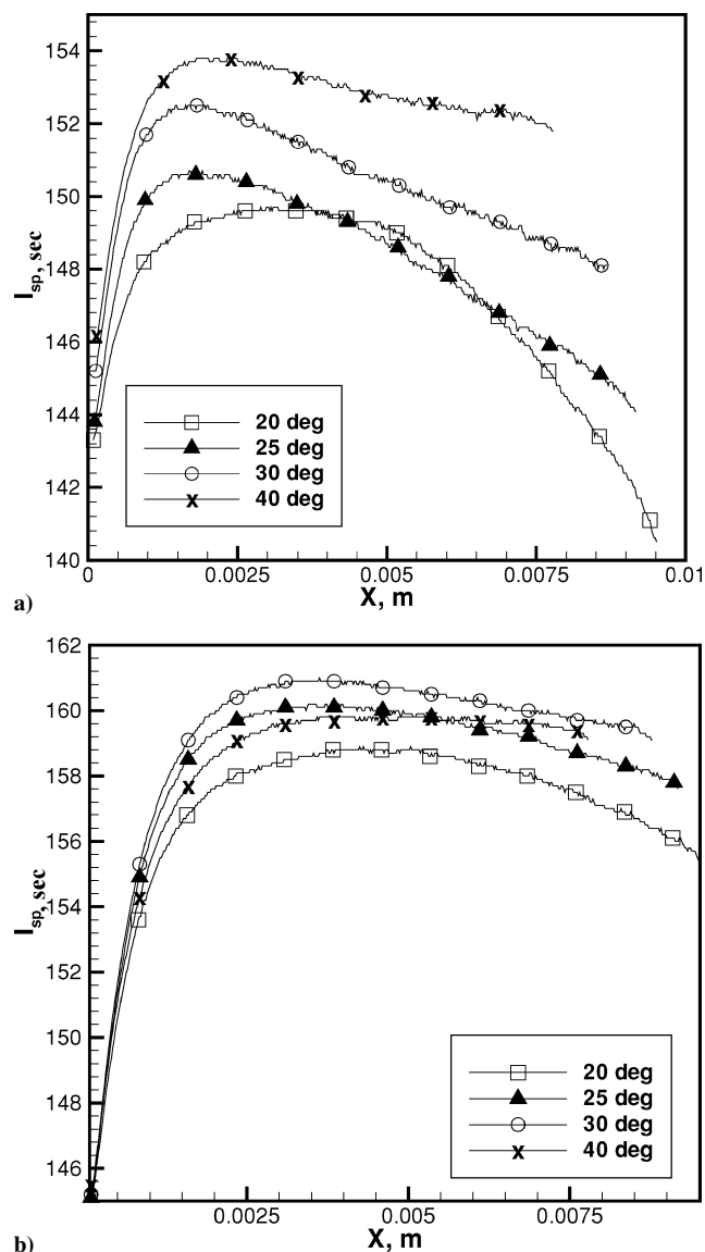
Fig. 15 Impact of the nozzle expansion angle on performance for helium: a) Re^* = 60 and b) Re^* = 200 .
