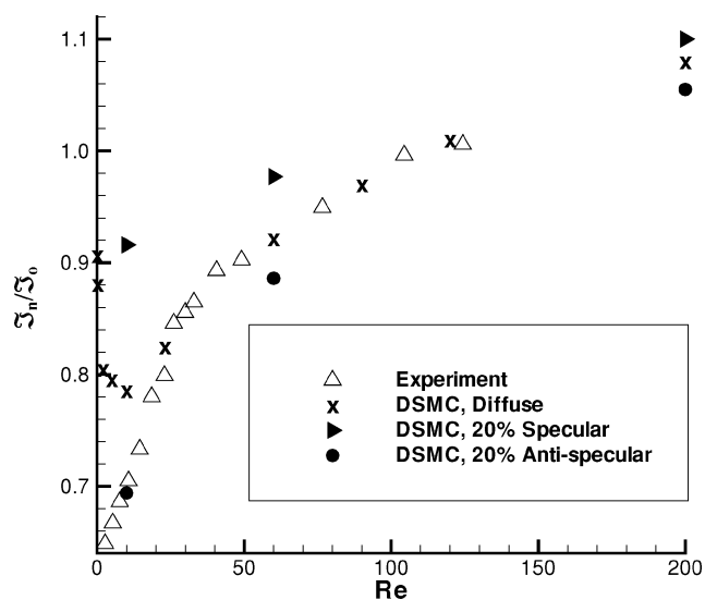
Fig. 12 Ratio of the nozzle to orifice thrust for helium as a function of Reynolds number.
