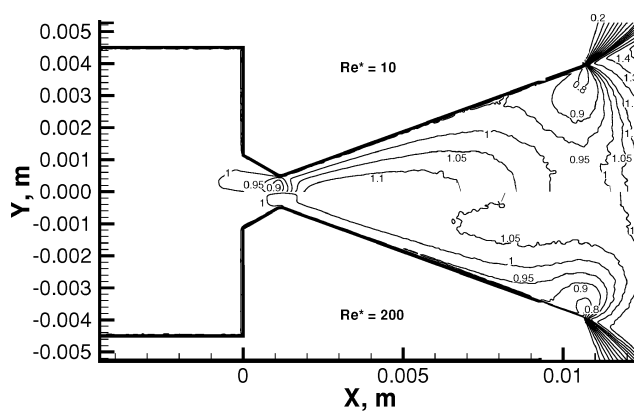
Fig. 7 Predicted T_x/T contours for helium flow inside the nozzle at Re^* = 10 (top) and 200 (bottom).
