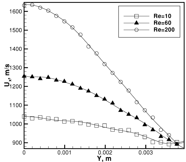
Fig. 9 Predicted axial-velocity profiles across the nozzle-exit plane for different Reynolds numbers for a helium flow. Y=0 corresponds to the symmetry axis.
