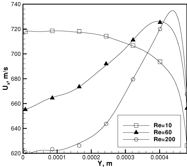
Fig. 8 Predicted axial-velocity profiles along the orifice plane for different Reynolds numbers for a helium flow. Y=0 corresponds to the symmetry axis.
