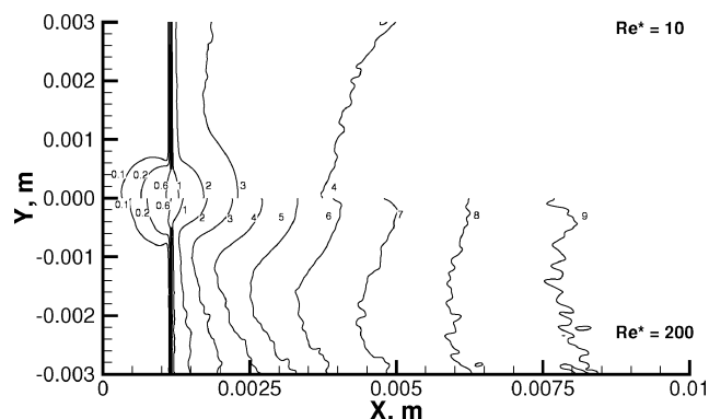
Fig. 4 Predicted Mach-number contours for helium orifice flow at Re^* = 10 (top) and 200 (bottom).
