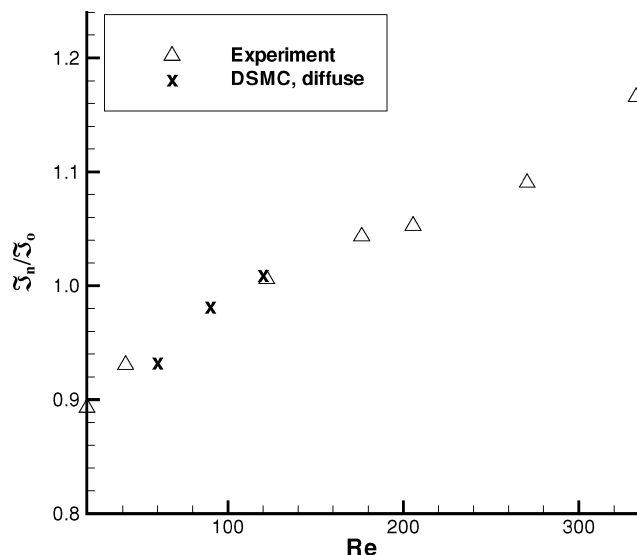
Fig. 13 Ratio of the nozzle-to-orifice thrust for nitrogen as a function of Reynolds number.
