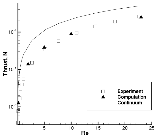
Fig. 11 Nozzle thrust comparison between experimental and numerical data for helium.
