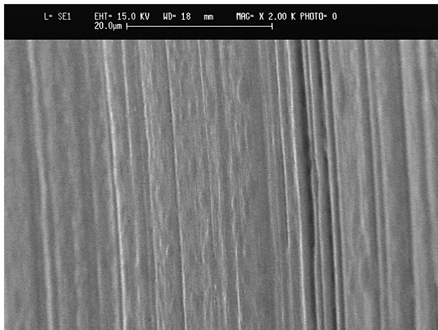
Fig. 3 Scanning electron microscope image showing the surface roughness of the expanding section of the conical nozzle.
