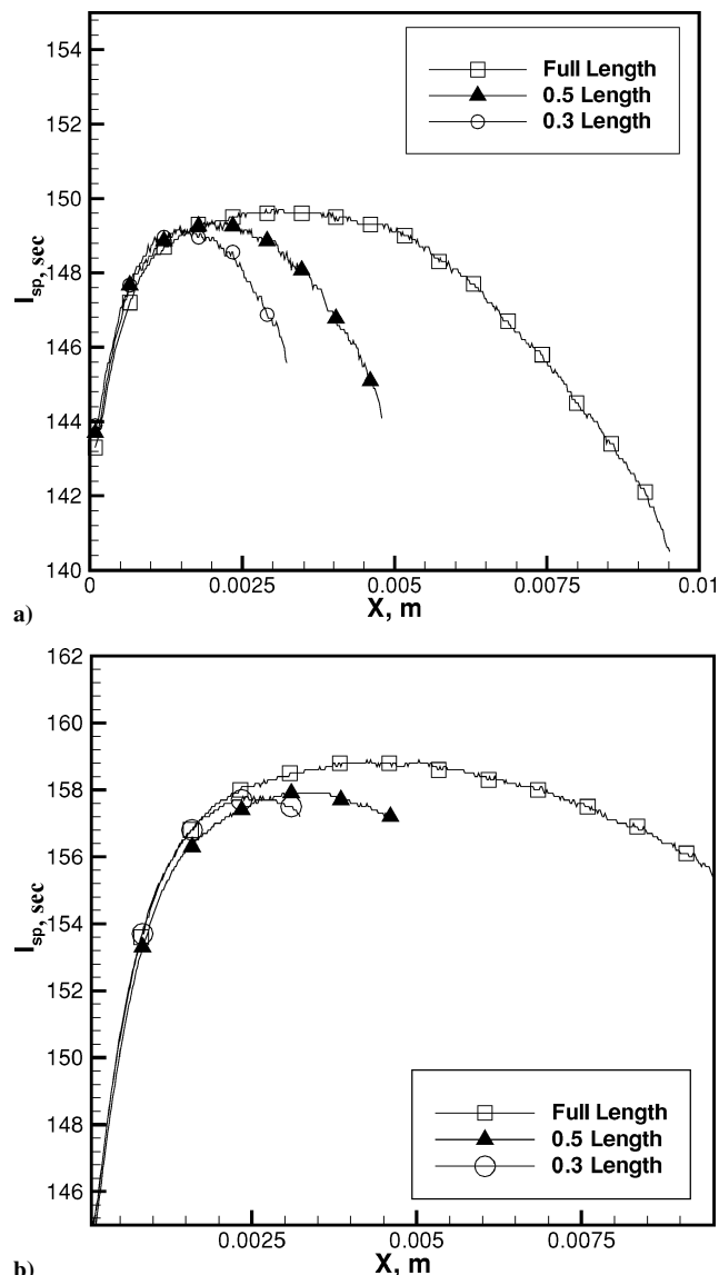
Fig. 14 Impact of the nozzle length on performance for helium: a) Re^* = 60 and b) Re^* = 200 .
