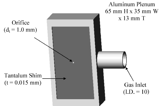
Fig. 1 Thin-walled orifice geometry.
