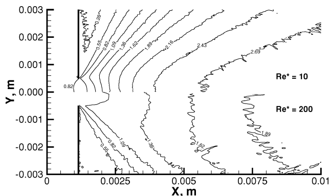
Fig. 6 Predicted T_x/T contours for helium orifice flow at Re^* = 10 (top) and 200 (bottom).
