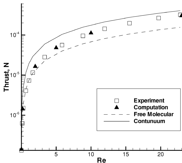
Fig. 10 Orifice thrust comparison between experimental and numerical data for helium.
