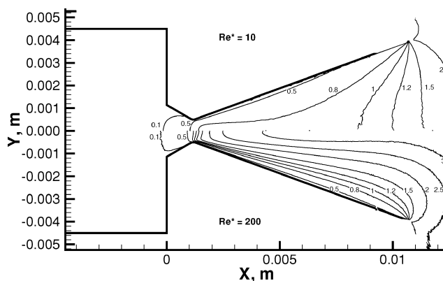
Fig. 5 Predicted Mach-number contours for helium flow inside the nozzle at Re^* = 10 (top) and 200 (bottom).
