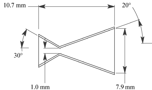
Fig. 2 Experimental geometry of the conical DeLaval nozzle.
